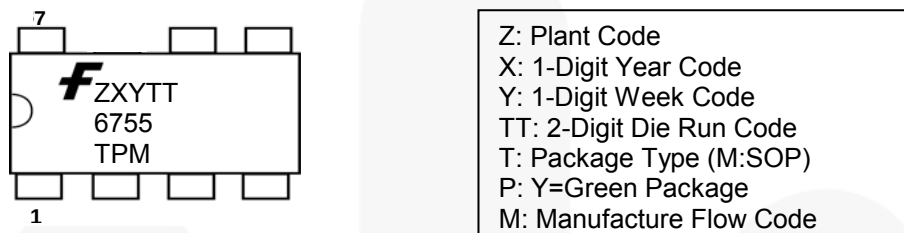
Figure 3. Top Mark
