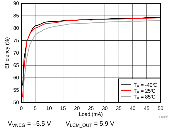
Figure 87. VNEG Efficiency
