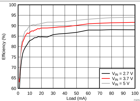
Figure 76. LCM Boost Efficiency
