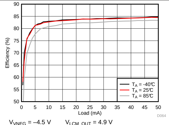
Figure 85. VNEG Efficiency
