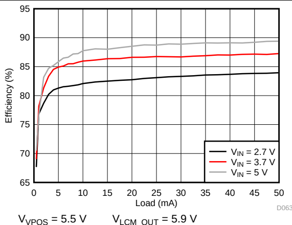
Figure 84. VPOS Efficiency
