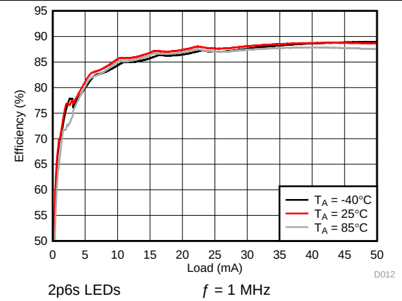
Figure 67. Backlight System Efficiency
