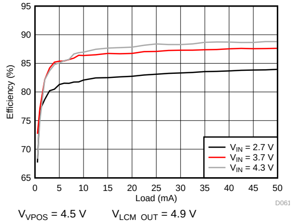
Figure 82. VPOS Efficiency
