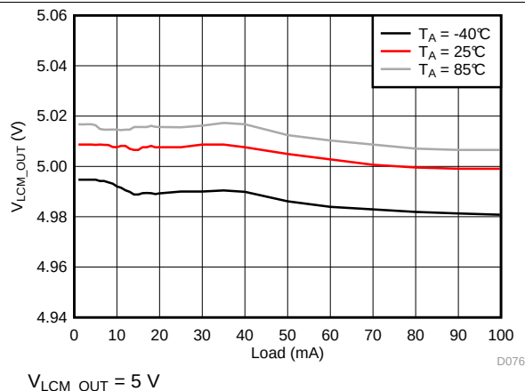
Figure 97. V_{LCM\_OUT} Load Regulation
