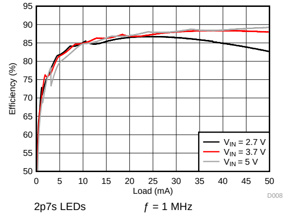
Figure 63. Backlight System Efficiency
