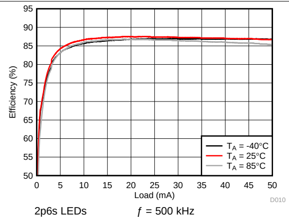
Figure 65. Backlight System Efficiency
