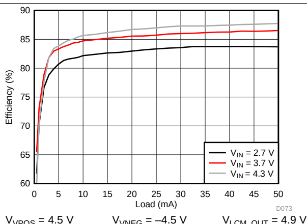
Figure 94. VPOS/VNEG Efficiency
