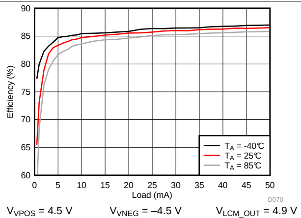
Figure 91. VPOS/VNEG Efficiency
