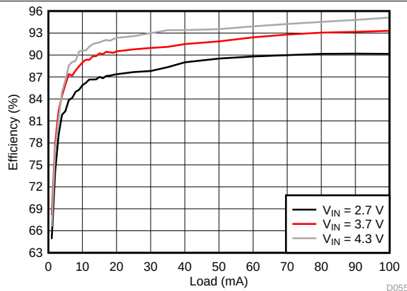
Figure 74. LCM Boost Efficiency
