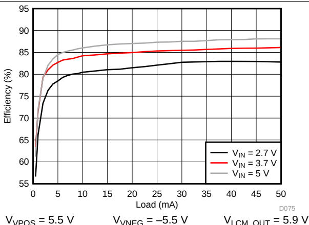
Figure 96. VPOS/VNEG Efficiency
