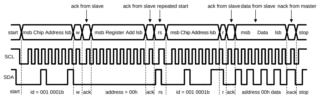
Figure 38. Register Read Format
