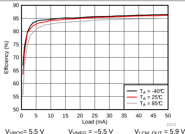
Figure 93. VPOS/VNEG Efficiency
