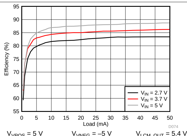
Figure 95. VPOS/VNEG Efficiency
