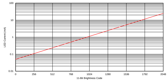
Figure 23. Response of LED Current vs Brightness Code on a Log Y Axis
