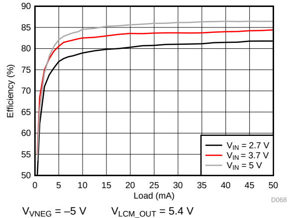
Figure 89. VNEG Efficiency
