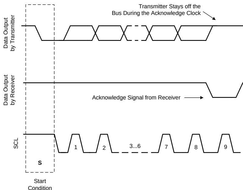
Figure 34. Acknowledge Signal
