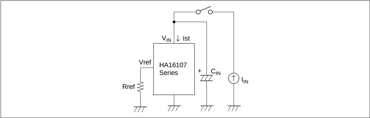
Figure 1 Standby Current Test Circuit
