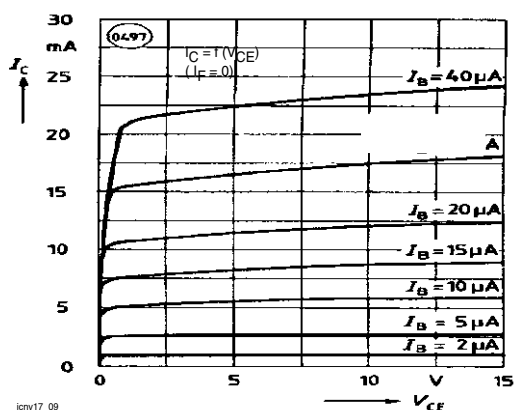
Figure 9. Transistor Characteristics
