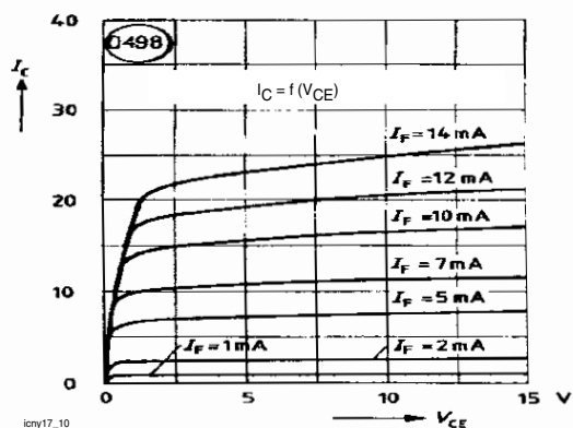
Figure 10. Output Characteristics
