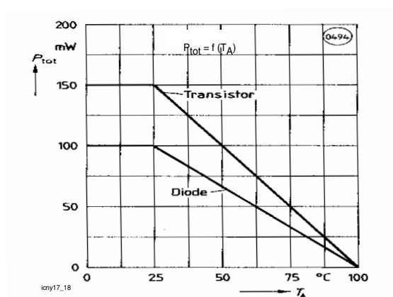
Figure 17. Permissible Power Dissipation for Transistor and Diode
