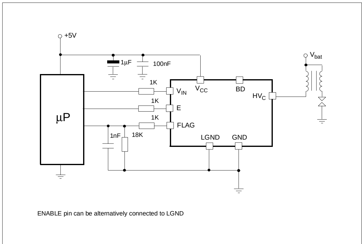
Figure 5: Typical application diagram
