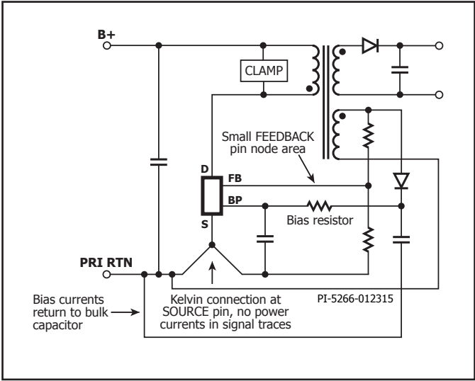
Figure 8. Schematic Representation of Recommended Layout With External Bias.
