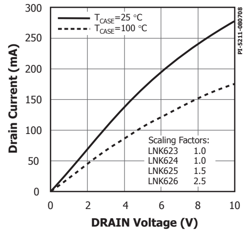
Figure 17. Output Characteristic.
